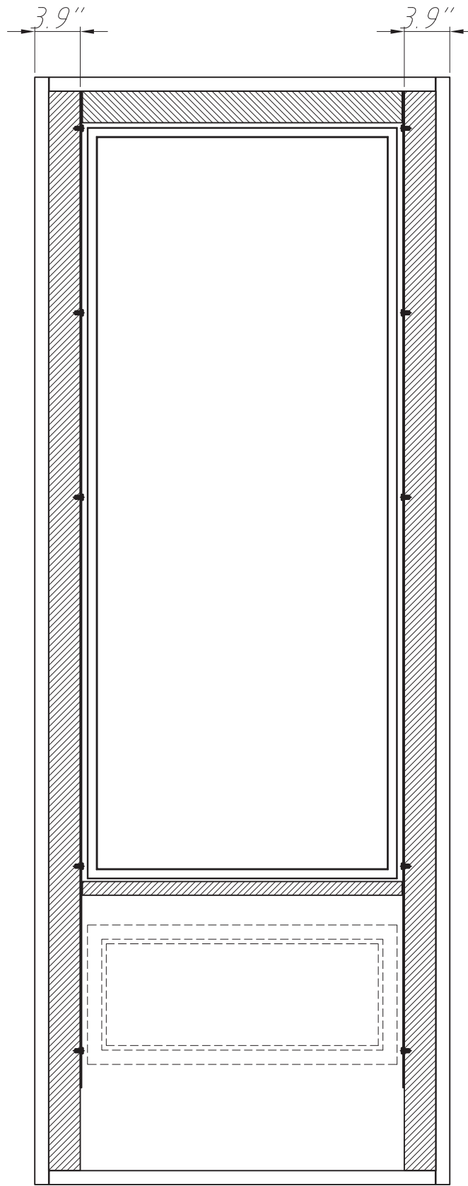
Lock Block Location Door Skin, Core and Glass Remove
