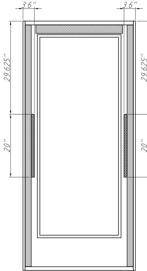
Lock Block Location Door Skin, Core and Glass Remove
